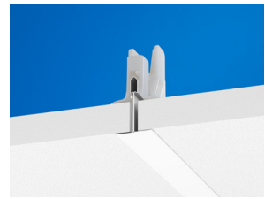
Connect T24 Main Runner C3 with Connect Hygiene Clip
