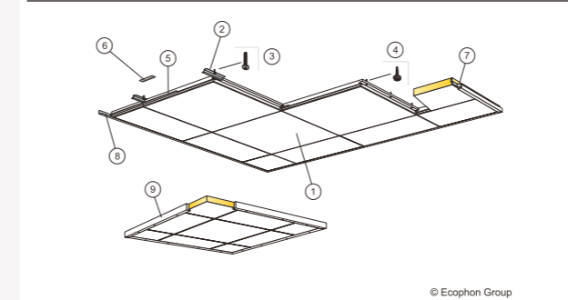
Installation diagram (M52) for Ecophon Master F
